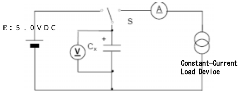
Measuring-Circuit
