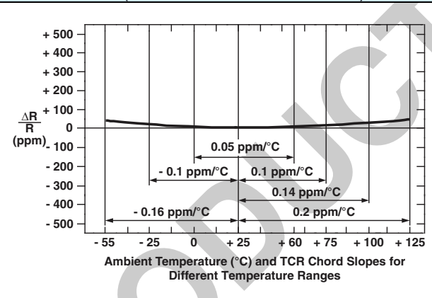
FIGURE 3 - TYPICAL RESISTANCE/TEMPERATURE CURVE
