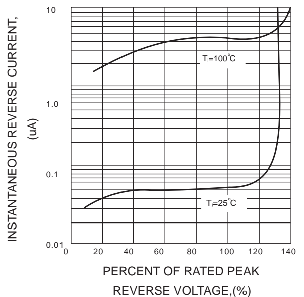
FIG.4-TYPICAL REVERSE CHARACTERISTICS
