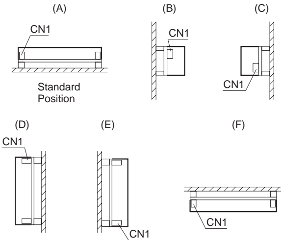
Fig.3.18 Mounting method
