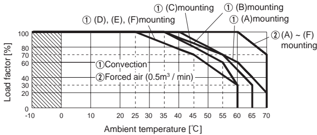
Fig.3.9 Ambient temperature derating curve (refer to Table 3.7)
