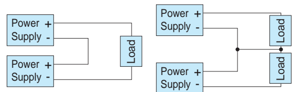
Fig.2.3 Examples of connecting in series operation
