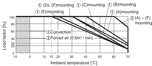
Fig.3.10 Ambient temperature derating curve (refer to Table 3.8)
