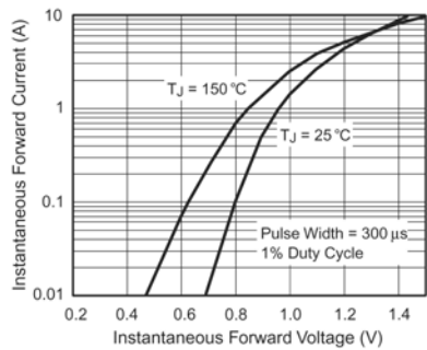
Figure 3. Typical Forward Voltage Characteristics Per Leg
