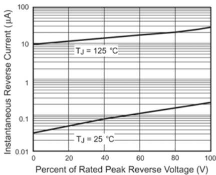
Figure 4. Typical Reverse Leakage Characteristics Per Leg
