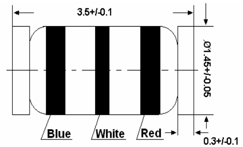
Glass case MiniMELF Dimensions in mm
