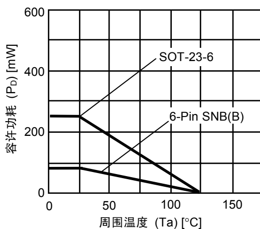
图4 封装容许功耗 (未安装时)
