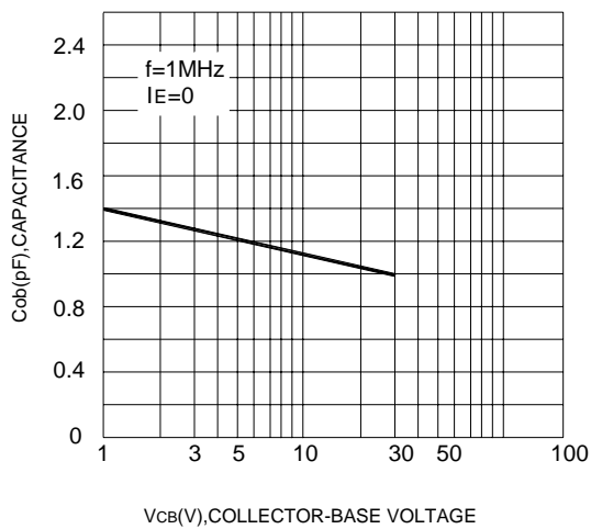
OUTPUT CAPACITANCE
