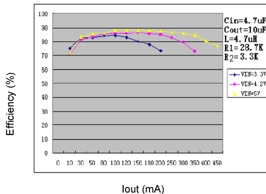
Figure 2. Efficiency Curve
