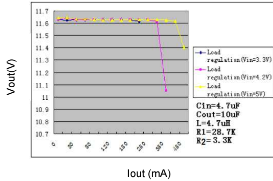
Load regulation
