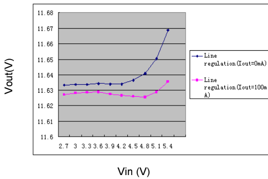
line Regulation
