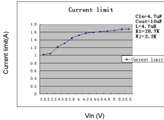
Current limit vs. Vin
