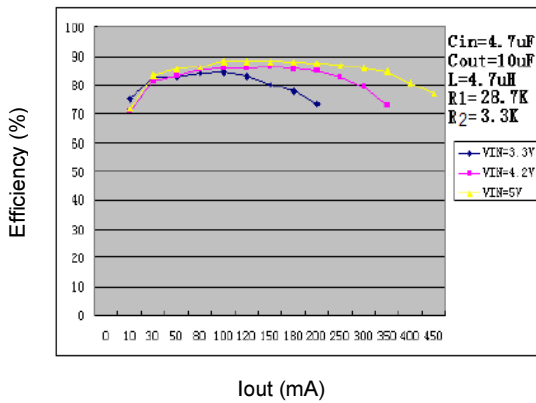
Efficiency Curve
