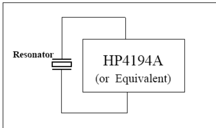
Figure 2. Measurement for Resonant Impedance
