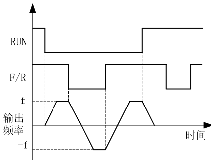
(b) F0.20=0, F0.05=0 运行正/反转逻辑
