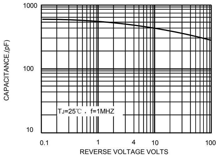
FIG.5-TYPICAL JUNCTION CAPACITANCE
