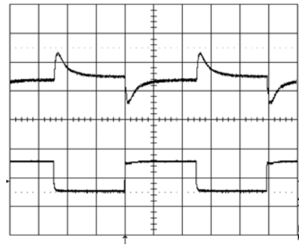
Output voltage response to load current step-change (0.5-1.5-0.5 A) at: T_{ref} = +25^\circ\text{C} , V_i = 27 V.
