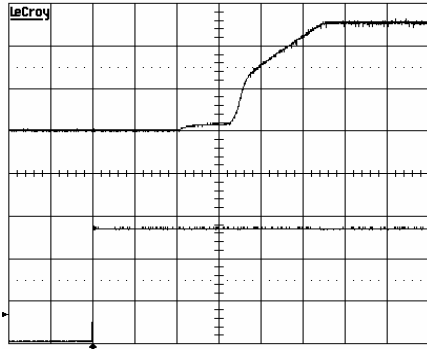
Start-up enabled by connecting V_i at: T_{ref} = +25^{\circ}C , I_o = 2 A resistive load, V_i = 27 V. Top trace: output voltage (2 V/div.). Bottom trace: input voltage (10 V/div.). Time scale: 1 ms/div..
