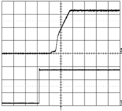
Start-up enabled by connecting V_i at: T_{ref} = +25^\circ\text{C} , I_o = 2 A resistive load, V_i = 27 V.
