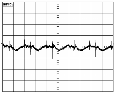
Output voltage ripple (5 mV/div.) at: T_{ref} = +25^{\circ}C , I_o = 2 A resistive load, V_i = 27 V. Time scale: 1 \mu s/div. See the filter in the Output ripple and noise section (EMC Specification).
