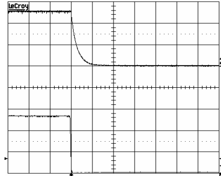
Shut-down enabled by disconnecting V_i at: T_{ref} = +25^{\circ}C , I_o = 2 A resistive load, V_i = 27 V. Top trace: output voltage (2 V/div.). Bottom trace: input voltage (10 V/div.). Time scale: 1 ms/div..
