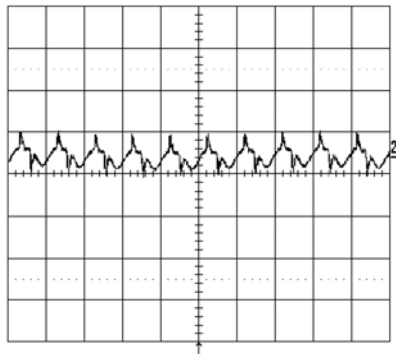
Output voltage ripple (5mV/div.) at: T_{ref} = +25^\circ\text{C} , I_o = 2 A resistive load, V_i = 27 V. Time scale: 2 \mu\text{s} /div.
