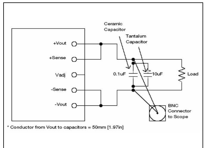
Output ripple and noise test setup
