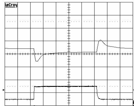
Output voltage response to load current step-change (0.5-1.5-0.5 A) at: T_{ref} = +25^{\circ}C , V_i = 27 V. Top trace: output voltage (200mV/div.). Bottom trace: load current (1 A/div.). Time scale: 0.1 ms/div.
