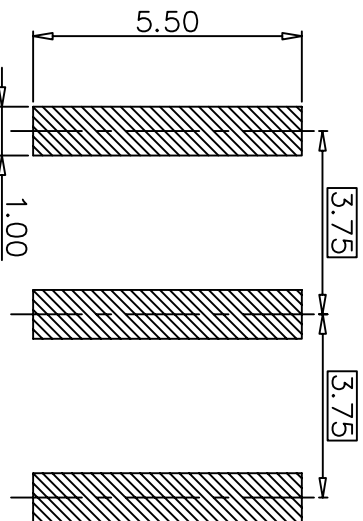
REFERENCE P.C.B. LAYOUT
