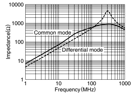
ACM1211-102-2PL
