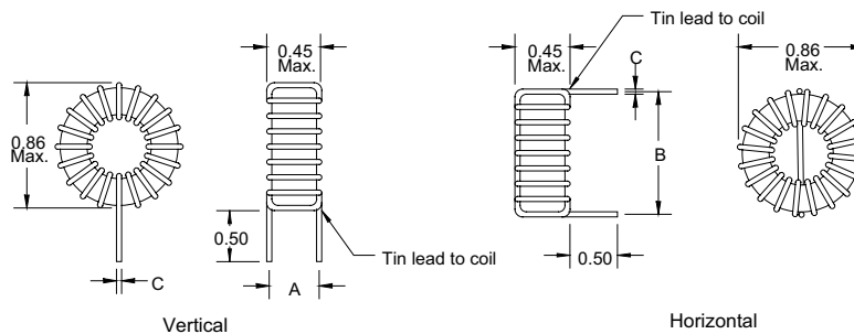
Dimensions: Inches
