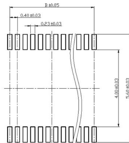
Recommended PC board pattern (mounting pad layout)
