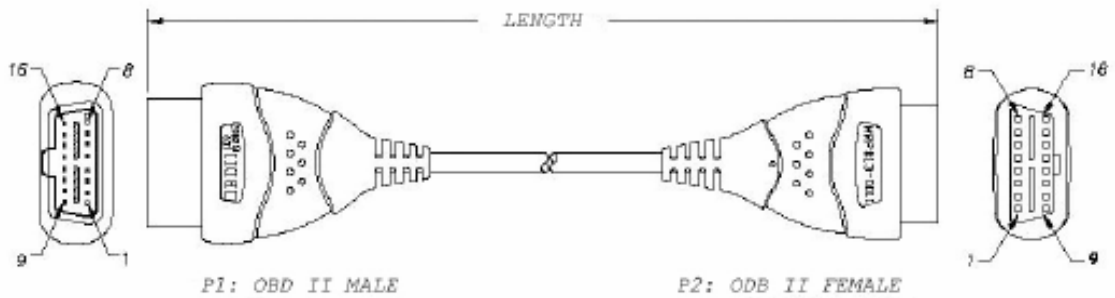
Kvaser OBD II Extension Cable
